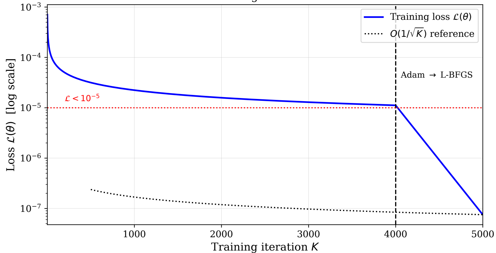
PINN Training Loss vs Iteration
